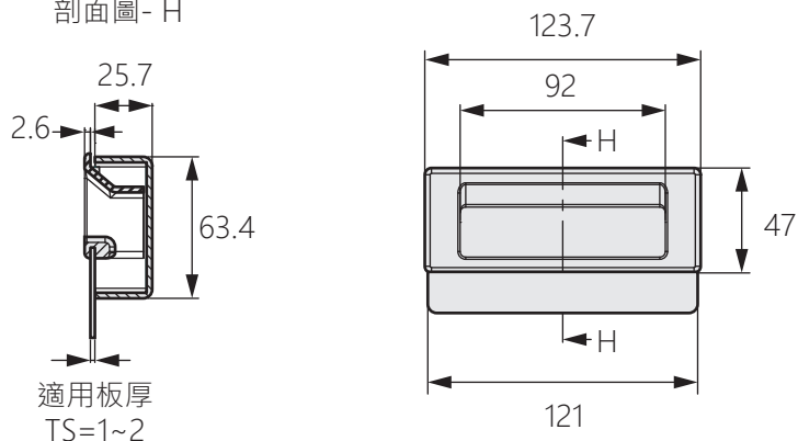
剖面圖-H
