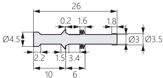
[JT-M5-Y]
