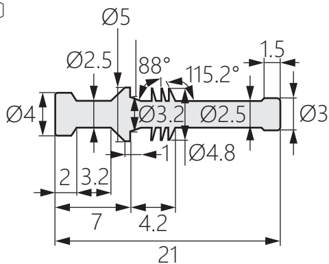
[JT-M4-Y]
