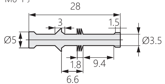
[JT-M6-Y]
