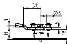
B型: 带圆形螺柱锁舌
