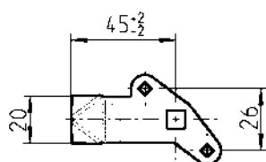
A型：带T型螺柱锁舌
