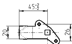
B型：带圆形螺柱锁舌
