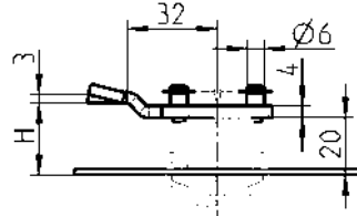
B型：带圆形螺柱锁舌
