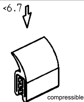
Sealing profile and clamping profile EPDM 60 ± 5 Shore A, black
