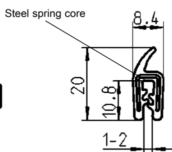
Sealing profile and clamping profile EPDM 60 ± 5 Shore A, black
