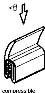
Sealing profile and clamping profile EPDM 60 ± 5 Shore A, black
